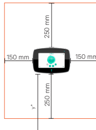
I-2.1: Mounting area
